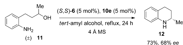
Scheme 2. Example of the intramolecular amination of alcohols.
