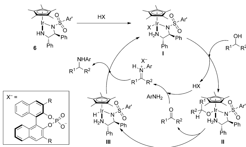
Scheme 3. Proposed catalytic cycle.
